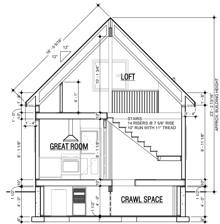
A CROSS SECTION 2 1/4" = 1'-0"
